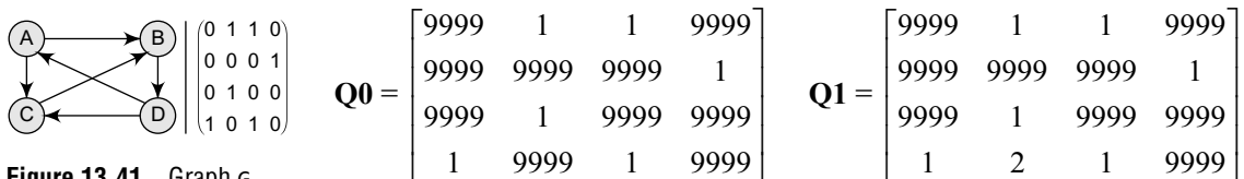
Figure 13.41 Graph G
